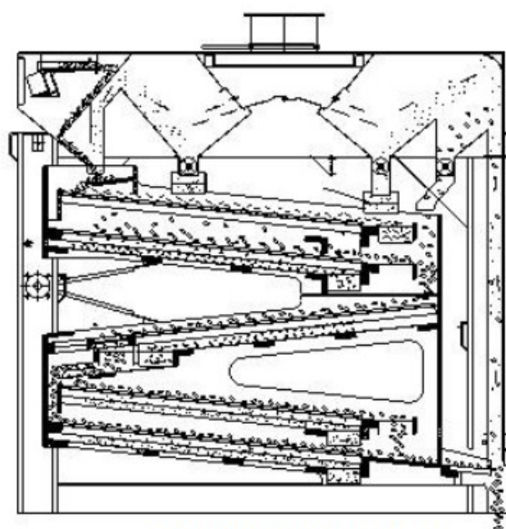
FCU WITH OPTIONAL VIBRATOR FEEDER
